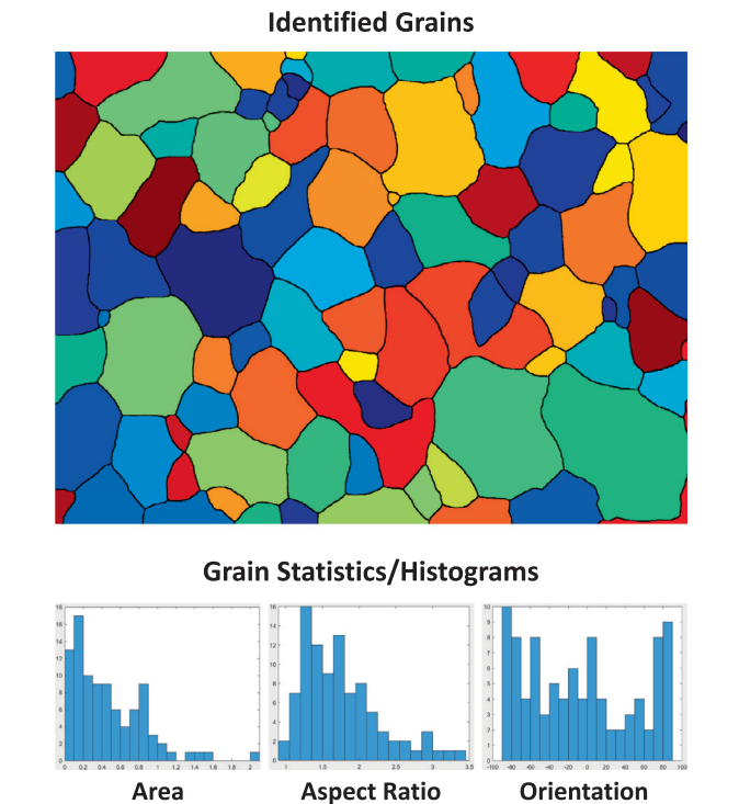
Fig. 11. Individual grains identified by our algorithm, and their statistics: histograms of grain areas, aspect ratios, and orientations.
